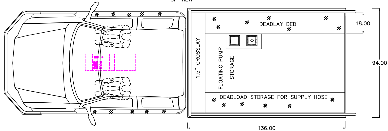
TOP VIEW
